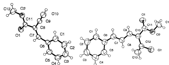
Figure 1. ORTEP representation of ( E )- 2e and ( Z )- 3i (right).
